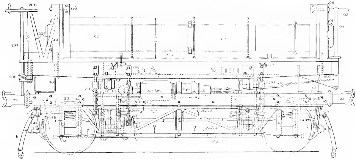
Fig. 336. Side Elevation.
